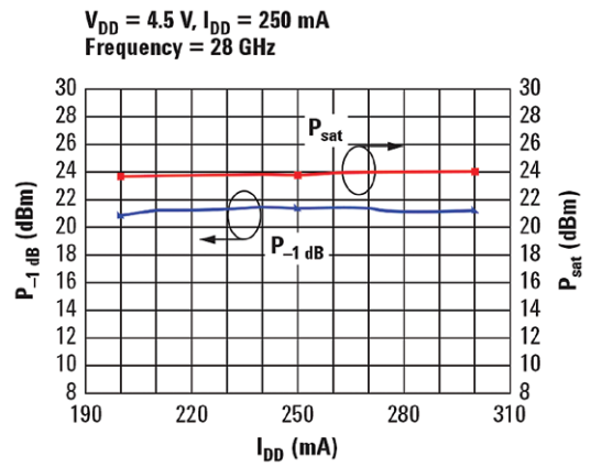
Figure 5. Output power vs. total drain current
