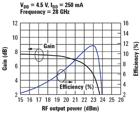
Figure 8. Gain compression and efficiency vs. power out
