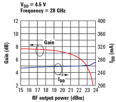
Figure 9. Gain and total drain current vs. output power
